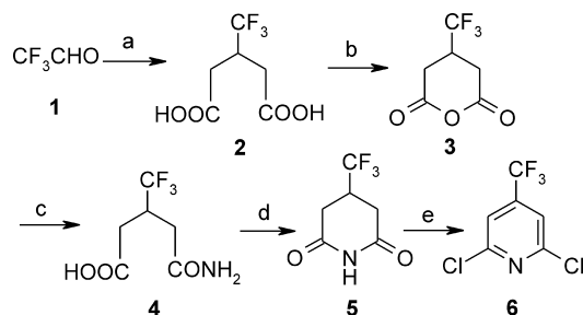
Scheme 1. Reagents and conditions: (a) cyanacetamide, EtOH, pyridine, rt, then 3 N HCl, reflux; (b) Ac 2 O, reflux; (c) NH 3 ·H 2 O, rt; (d) 220–230 °C, 1.5 h; (e) POCl 3 , reflux, 10 h.
