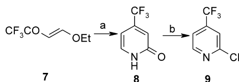
Scheme 2. Reagents and conditions: (a) ClCH 2 CN, Zn, TMSCl, THF, 3 h, concn HCl, reflux; (b) POCl 3 , PCl 5 , 3 h.
