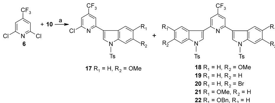
Scheme 4. Reagents and conditions: (a) Pd(PPh 3 ) 4 , Na 2 CO 3 , benzene, MeOH.
