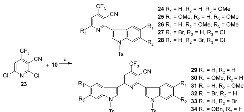
Scheme 5. Reagents and conditions: (a) Pd(PPh_3)_4 , Na_2CO_3 , benzene, MeOH or DME.
