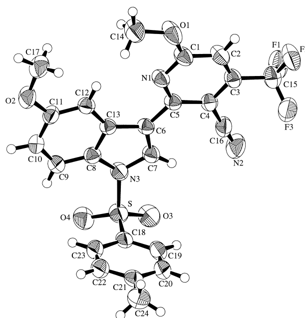
Figure 2. ORTEP drawing of the X-ray crystal structure of compound 25 .
